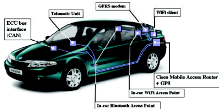
▲ Figure 2: Embedded architecture
